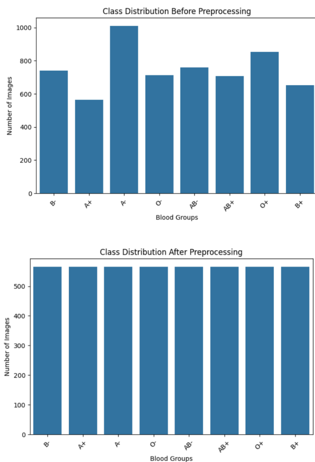
Fig. 1. Class distribution before and after preprocessing
